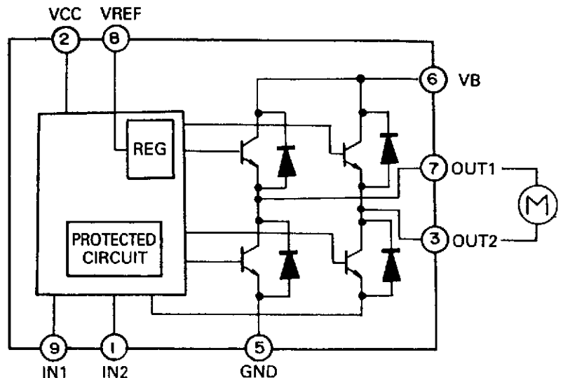
2. Block Diagram
